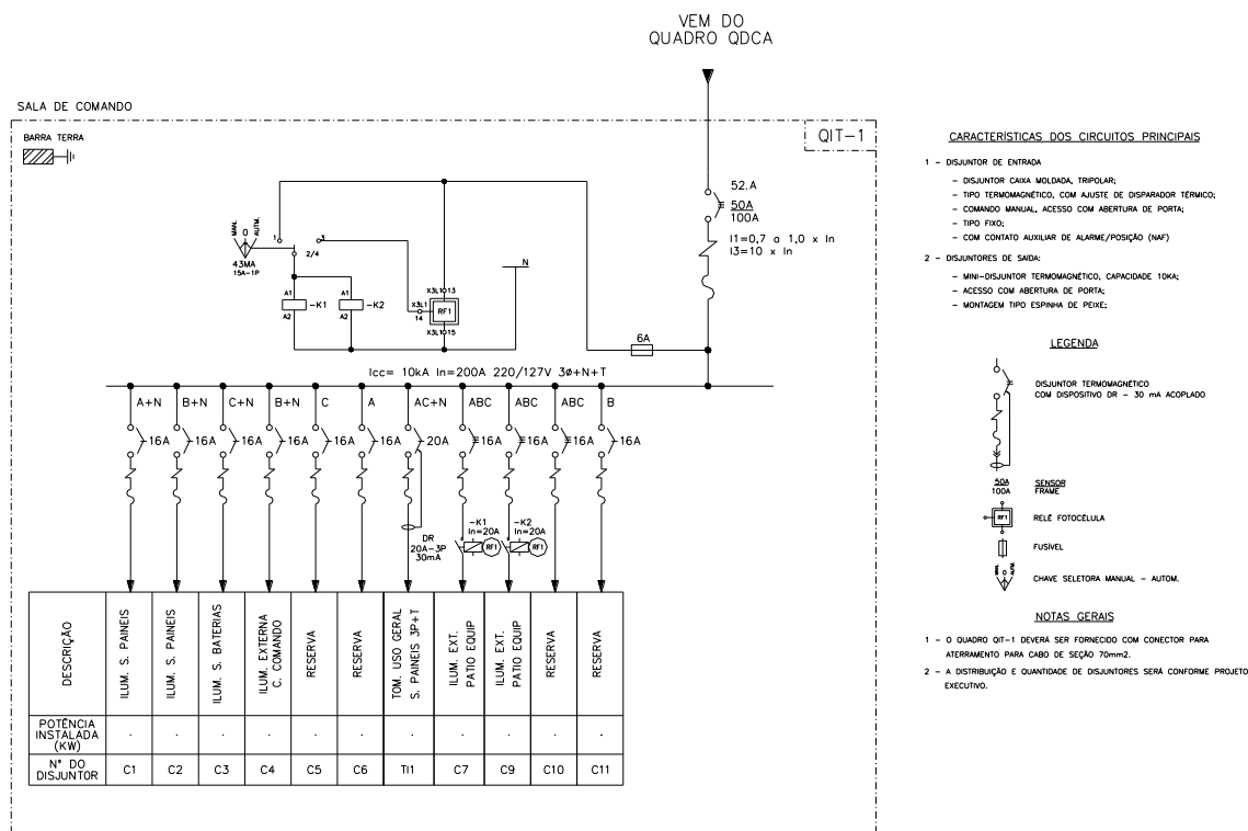
Figura 22 - Unifilar painel QIT-1
