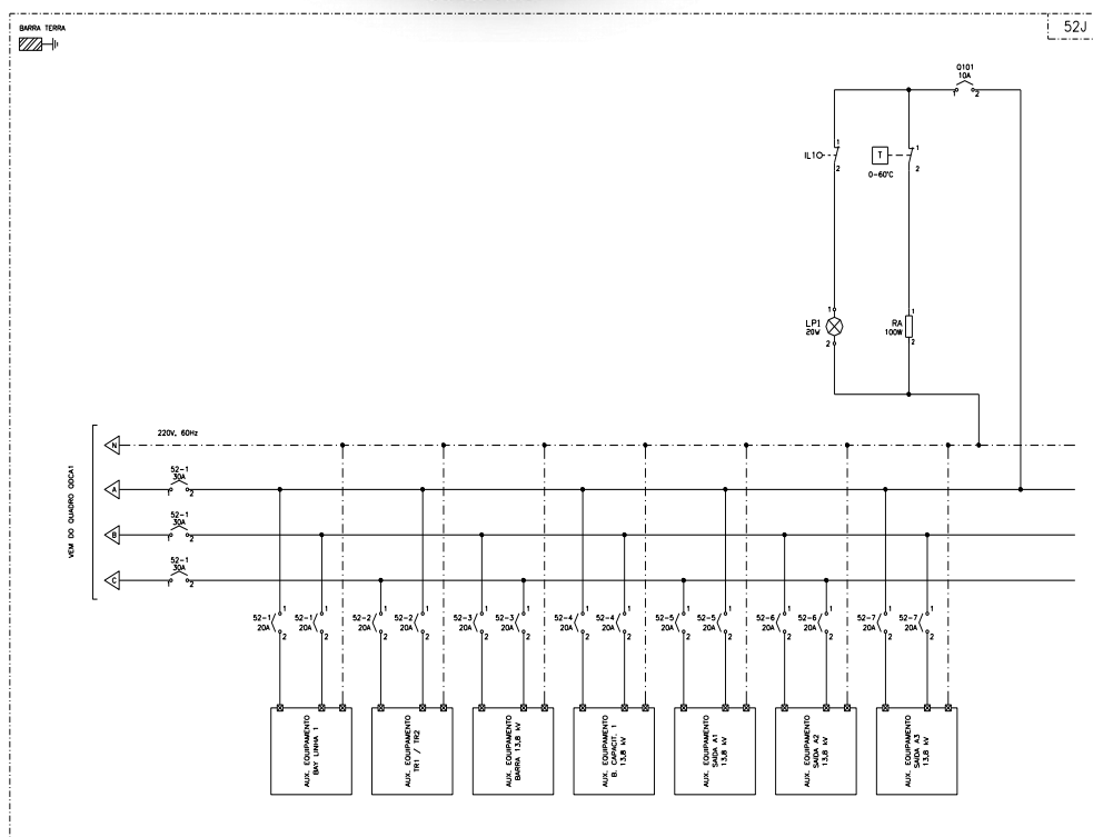
Figura 18 - Unifilar painel 52J
