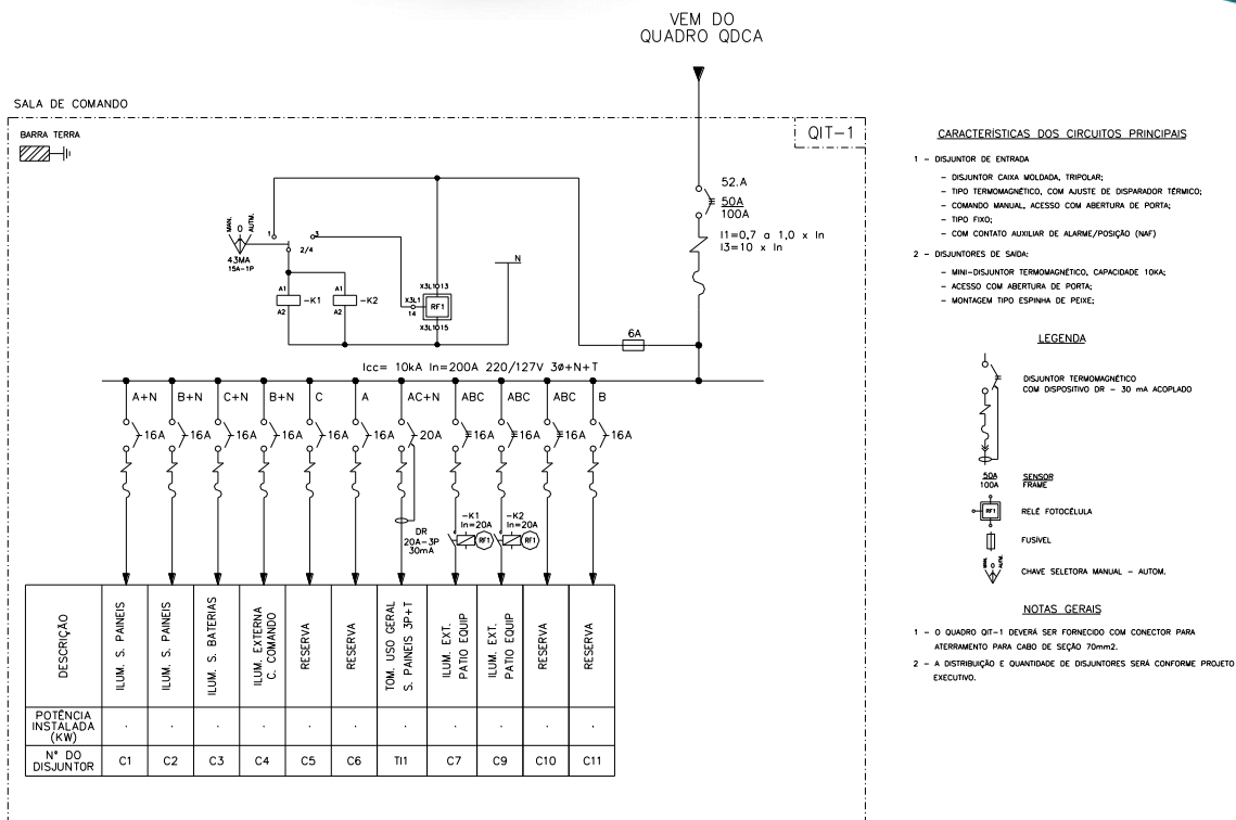
Figura 17 - Unifilar painel QIT-1
